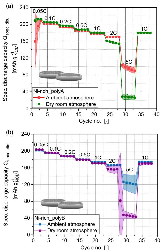
Figure 1. Specific discharge capacity of lithium metal/NCM coin cells. a) Ni-rich_polyA cathodes and b) Ni-rich_polyB cathodes produced in ambient or dry-room atmosphere.
