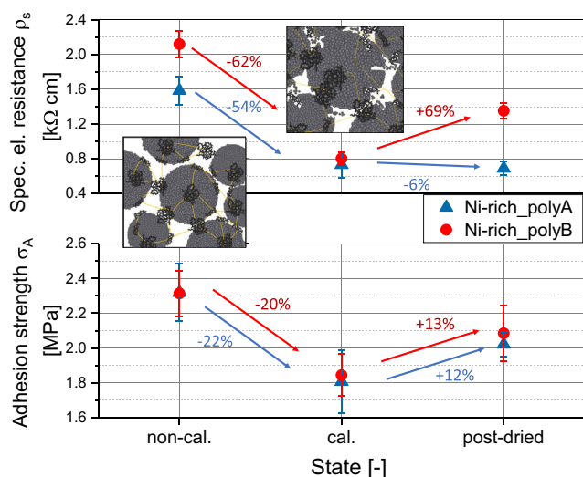
Figure 6. Specific electrical resistance and adhesion strength at different process steps of the Ni-rich cathodes.
