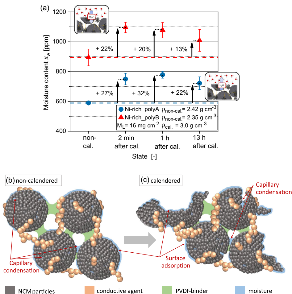
Figure 2. Top: a) moisture content of the Ni-rich_polyA and Ni-rich_polyB cathodes before and after calendaring (cal.) determined by Karl–Fischer Titration. Bottom: schematic illustration of water adsorption in an NCM-based cathode in b) non-calendered and c) calendered state (Adapted by permission from Ref. [32], Copyright (2021) IOP Publishing, CC BY 4.0).
