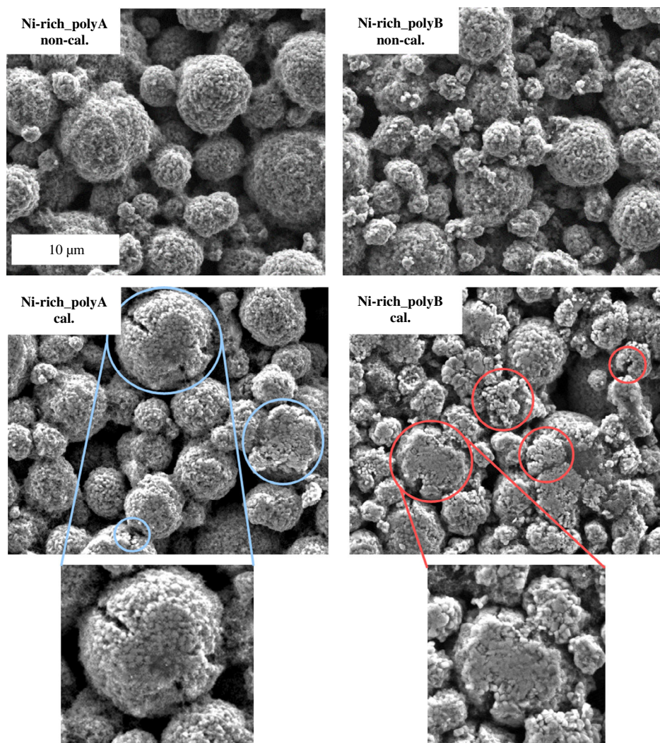
Figure 5. Scanning electron microscope (SEM) images of non-calendered and calendered Ni-rich_polyA and Ni-rich_polyB cathodes with a magnification of 4400 \times . Examples of particle breakage and cracking are marked by cycles.
