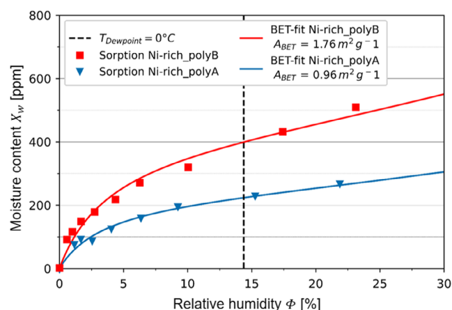
Figure 3. Sorption isotherms of Ni-rich_polyA and Ni-rich_polyB cathodes in non-calendered state obtained from magnetic suspension microbalance measurements ( 30^\circ\text{C} ).
