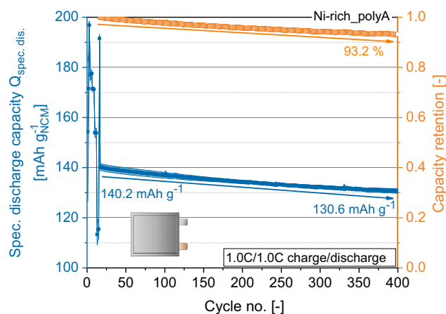
Figure 10. C-rate testing and long-term cycling (1.0C/1.0C charge/discharge) of graphite/NCM pouch cells with the Ni-rich_polyA cathode.
