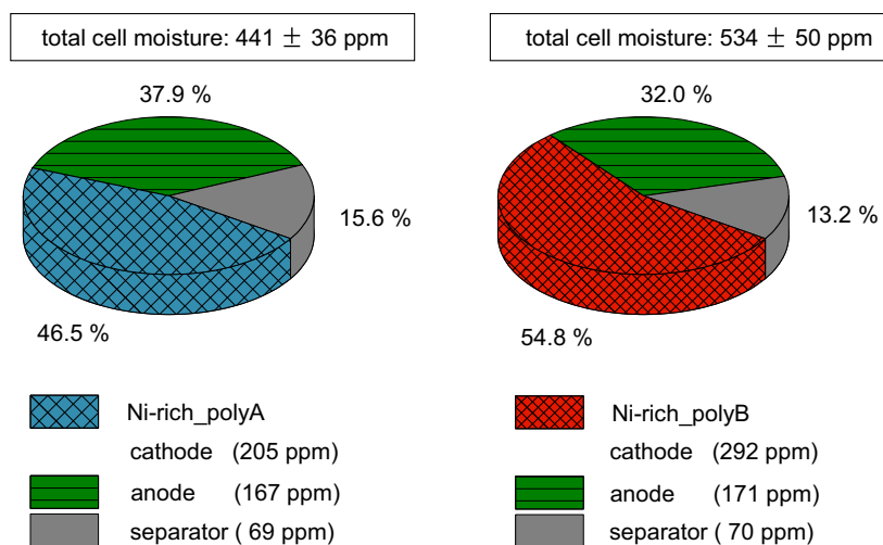
Figure 7. Total cell moisture of the single-compartment pouch cells after post-drying, with indication of the moisture amounts of each cell component, calculated according to the mass ratios of the cell components without current collectors.
