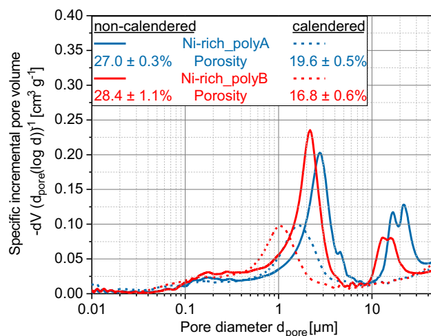
Figure 4. Pore-size distribution of the non-calendered and calendered Ni-rich_polyA and Ni-rich_polyB cathodes. Target coating density of the calendered cathodes: \rho_{\text{C}} = 3.0\text{ g cm}^{-3} .
