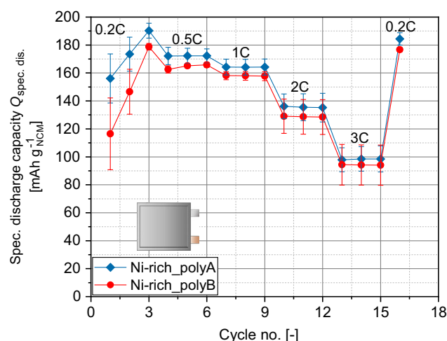
Figure 8. C-rate testing of lithium-ion battery (LIB) graphite/NCM pouch cells with Ni-rich_polyA and Ni-rich_polyB cathodes. Charging rate was set to 0.2C.
