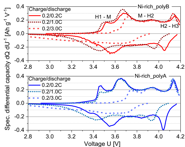
Figure 9. Specific differential charge and discharge capacity versus voltage of Ni-rich_polyA and Ni-rich_polyB full-pouch cells at different C-rates during discharge (0.2C, 1C, 3C). For each C-rate, the third cycle is demonstrated.
